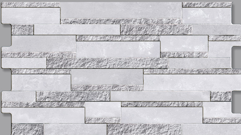
Pacific Ocean - 09
