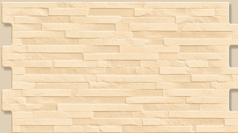
Antarctica - 15
